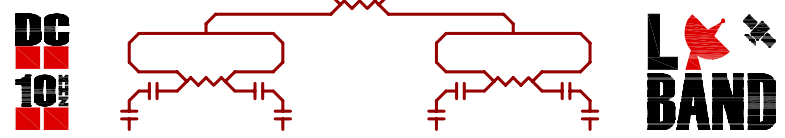
4-way L-band power splitter; DC & 10 MHz block 4 ports. Typically used splitting an LNB signal to 4 receivers where the output DC and 10 MHz must be blocked.
